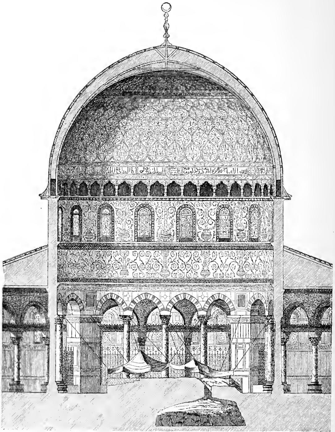
FIG. 192.—SECTION OF THE SAKHRA MOSQUE AT JERUSALEM.
